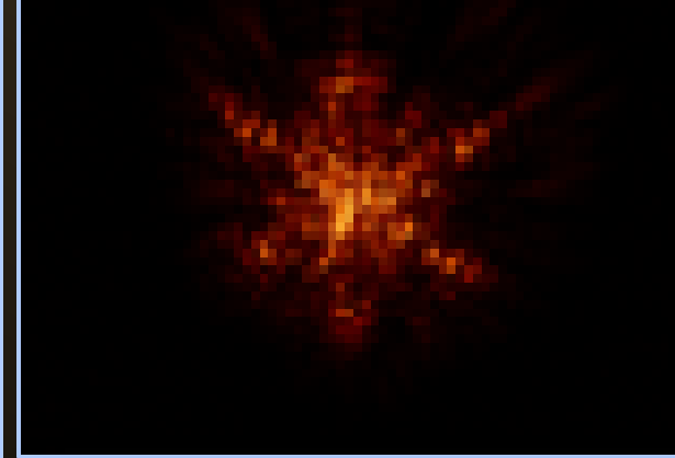
ROMAN- First image of a point source (pre-optical alignment, in-air)
