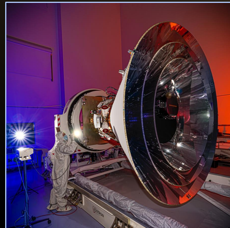
SPHEREx observatory in a horizontal position, showing all three layers of photon shields as well as the telescope. Credit: BAE Systems, Courtesy NASA/JPL-Caltech.
