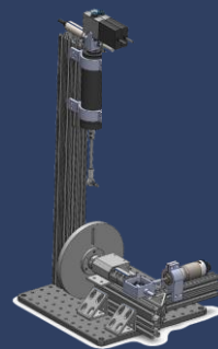
Deep Subsurface Drill Concept
