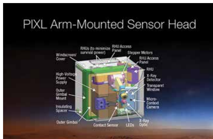
Planetary Instrument for X-Ray Lithochemistry (PIXL)
