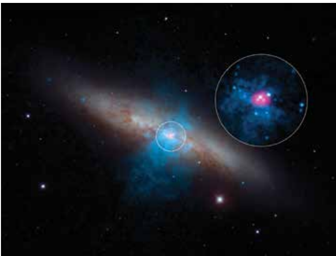
NuSTAR spotted a pulsing of X-rays streaming from the ultraluminous X-ray source M82 X-2 (magenta), discovering the brightest pulsar found to date. This image combines data from three telescopes: visible light from National Optical Astronomy Observatory's 2.1-meter telescope at Kitt Peak, AZ (starlight is white, lanes of dust appear brown), low-energy X-ray data from NASA's Chandra X-ray Observatory (blue), and higher-energy X-ray data from NuSTAR (pink). (Image credit: NASA/JPL-Caltech/SAO/NOAO)
