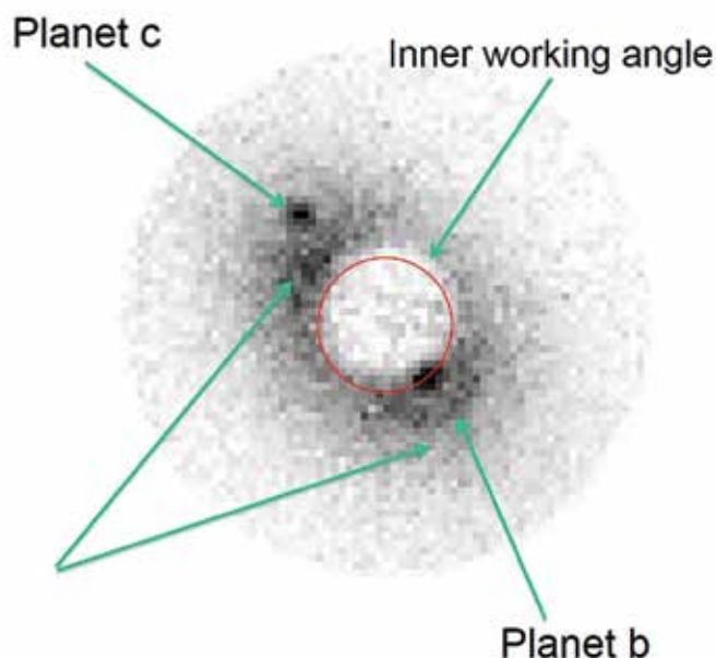
Simulated WFIRST-AFTA coronagraph image of the 47 UMa planetary system, including planets and the exozodiacal disk. The WFIRST-AFTA coronagraph will provide the first reflected-light visible images of the planetary systems of nearby stars.
