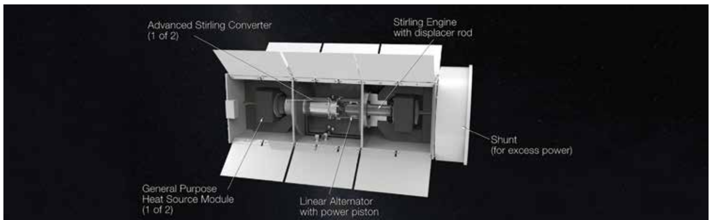
Radioisotope generator based on the free-piston Stirling converter design developed by Sunpower, Inc. The device is approximately 0.3m long. (Image Credit: NASA JPL)
