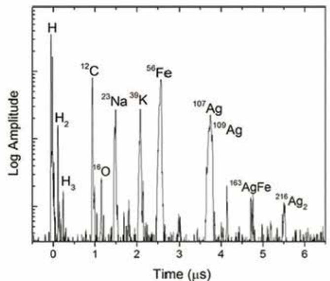
A sample mass spectrum measured by the NDA instrument using the dust accelerator facility at the University of Colorado.
