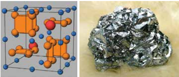
Left: Skutterudite crystal structure. Right: naturally occurring (Fe,Co,Ni)As 3 ore found in the Skutterud mine in Norway. (Image Credit: Thierry Caillat/NASA JPL)
