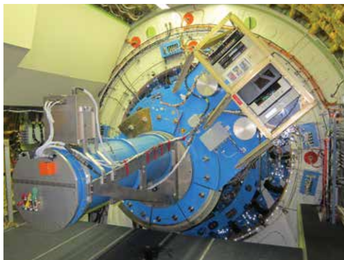
EXES mounted onboard SOFIA (Image credit: NASA/SOFIA/EXES/Mathew Richter)
