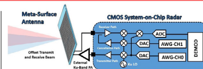
Block diagram of the CMOS SoC radar chip with the meta-surface antenna.
