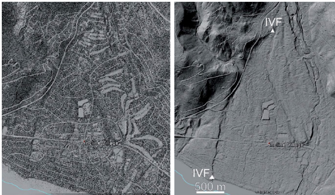
FIGURE 2-2. Shaded relief of full feature (all lidar returns in left) and bare earth (right) of the area around Incline Village, Nevada, in the north Lake Tahoe area. Fault scarps and fluvial features along the Incline Village Fault (IVF) are marked by white triangles. Data provided by Tahoe Regional Planning Agency ( http://dx.doi.org/10.5069/G9PN93H2 ; figure from Donnellan et al., 2016). High-resolution lidar-derived topographic data available from OpenTopography ( www.opentopography.org ; Crosby et al., 2011).
