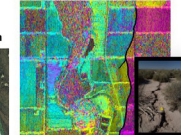
Apr 4, 2010 M 7.2 Baja California Earthquake
