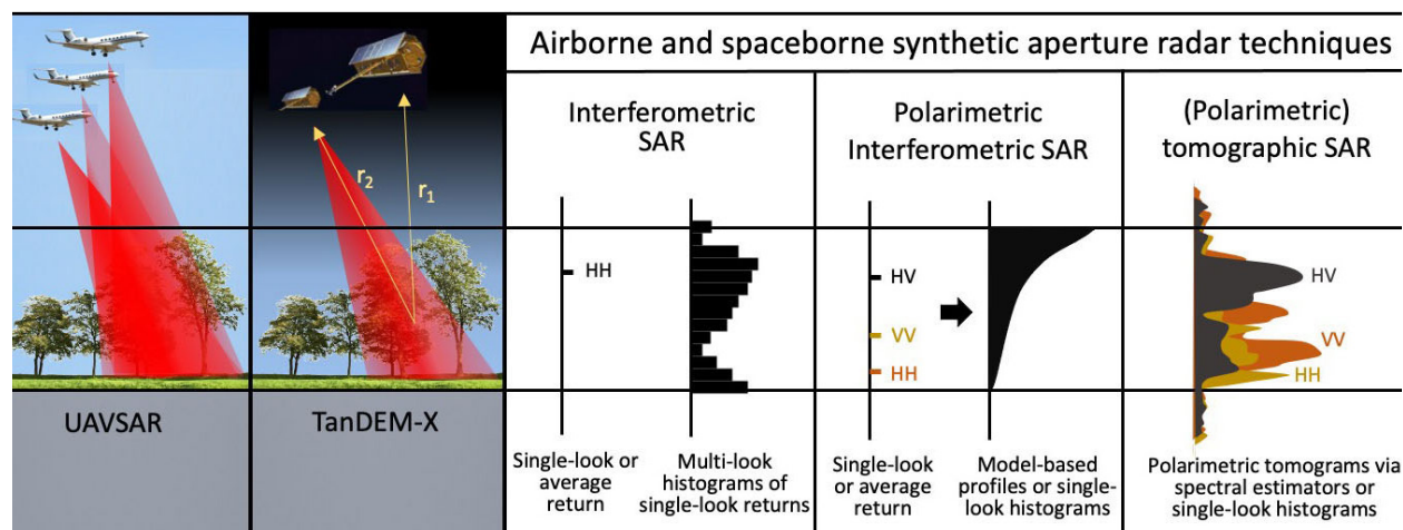
FIGURE 4-2. Examples of current airborne and spaceborne systems for STV mapping with associated InSAR, PolInSAR and TomoSAR measurements approaches.
