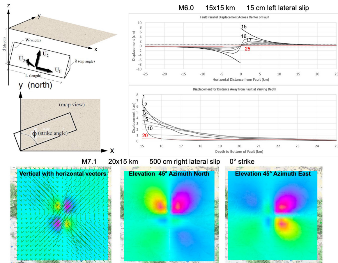
FIGURE 6-1. Example sensitivity models for dislocations in an elastic half space. Model parameters are noted in the top left diagram. Top right shows model output for a M6.0 earthquake. The top model shows displacements perpendicular to a vertical strike slip fault. Dotted horizontal line marks an example 0.5 cm displacement threshold. Deformation would not be detectable for a depth of 25 km for the bottom of the fault. Plotting depth of fault versus displacement profiles for various distances away from the fault shows how the deformation spreads out for deeper faults and is not detectable more than 20 km away from the fault. The bottom panels show simulated images for different line of sight components. Observed deformation is sensitive to the orientation of the fault and the line-of-sight direction for an InSAR instrument.
