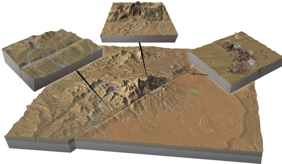
FIGURE 3-1. Actively deforming plate boundary zones contain active faulting and landslides. High-resolution topography is needed to measure past activity and in response to present-day activity.
