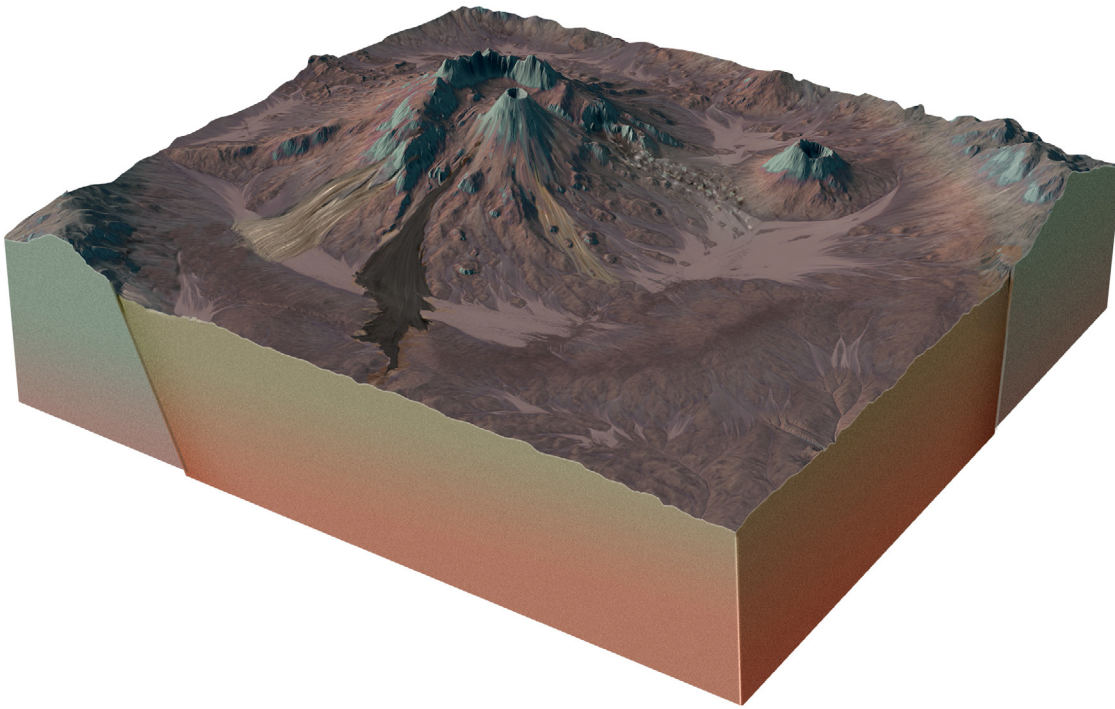
FIGURE 3-2. Volcanoes are capable of large changes in topography, from edifice-scale caldera formation to active lava flows, dome extrusion, and pyroclastic flows and secondary landslides.
