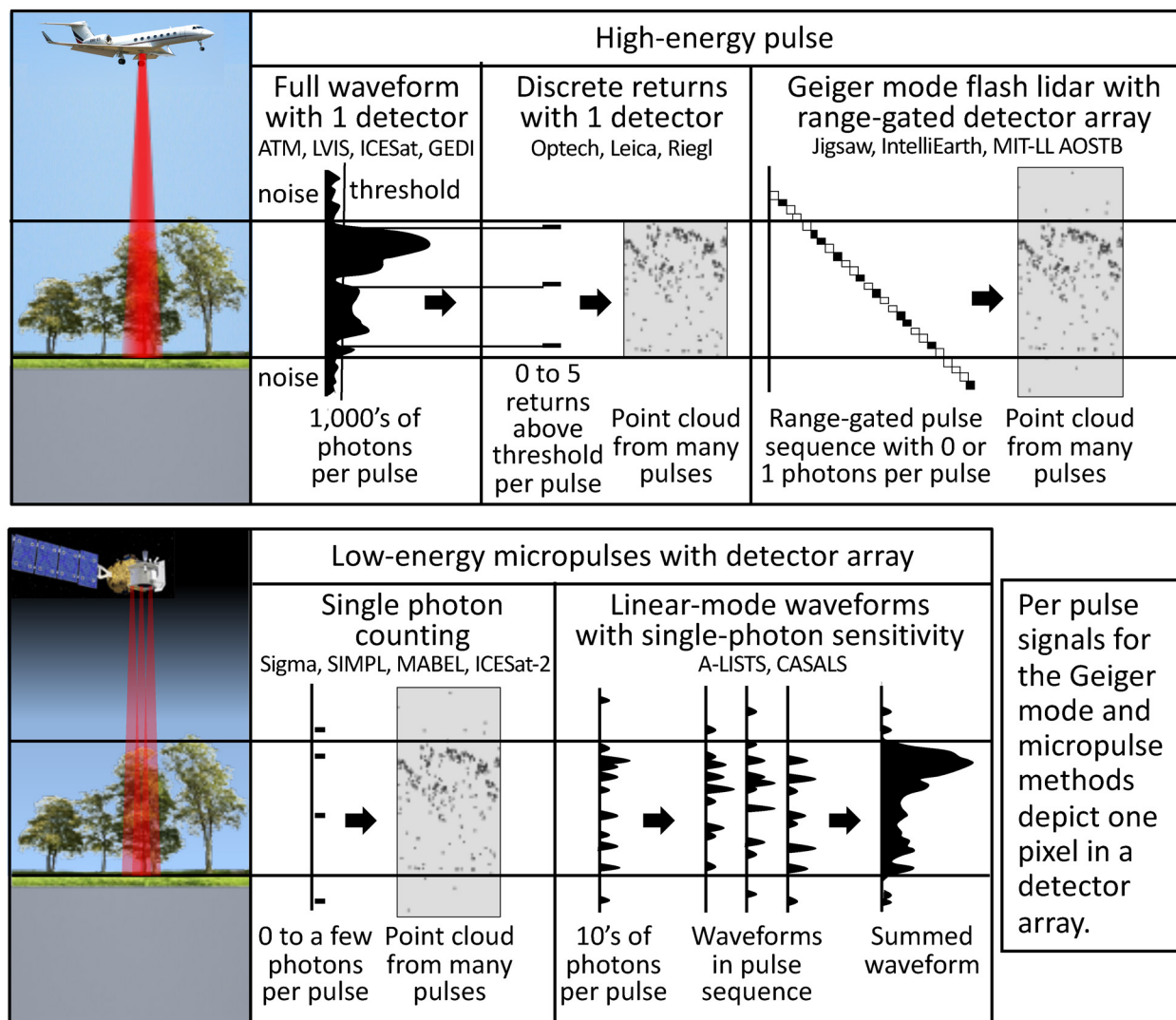
FIGURE 4-1. Lidar measurement approaches are divided into methods using single, high-energy laser pulses and those using high-repetition, low-energy micropulses.
