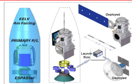
Example of instrument miniaturization leading to ESPA-class payload
